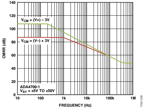
Figure 37. Common-Mode Rejection Ratio (CMRR) vs. Frequency, V SY = ±5 V to ±50 V
